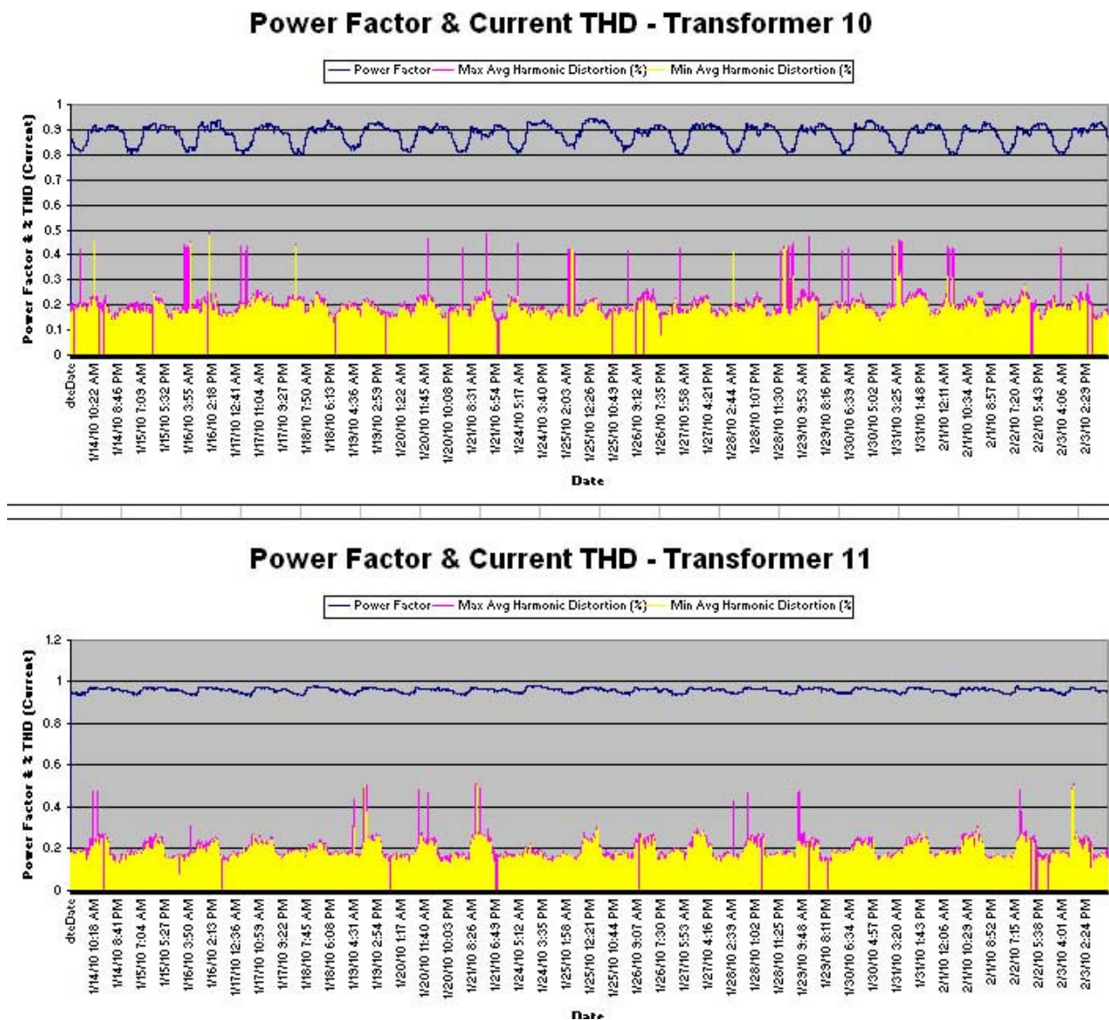
Figure 11 – Power Factor of Two Transformers that share a primary. The apartments attached to transformer 11 have had the power factor raised. Nothing has been done to the apartments attached to transformer 10
