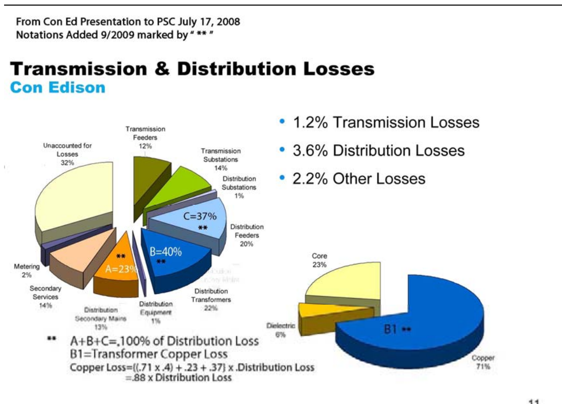
Figure 1: Excerpted from Transmission and distribution Losses. Consolidated Edison. Originally presented July 17, 2008 Percentage Notations added September, 2009.
