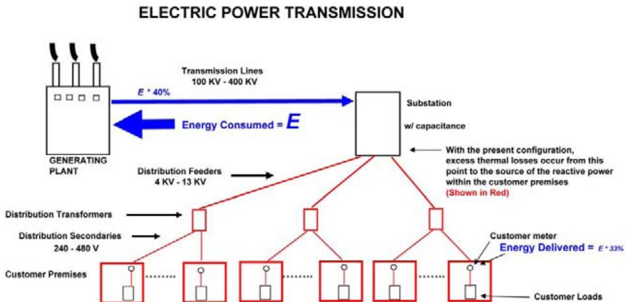
Figure 4 – Block diagram of the electric power transmission system. At present, the utilities correct reactive power at the substations. The distribution system, shown in red, operates with a less than optimal power factor. “At Load” power factor correction will reduce the losses on that entire part of the system.
