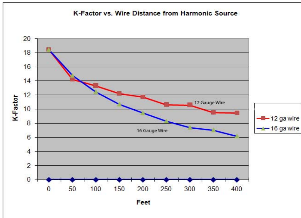
Figure 16 - K-Factor versus distance from the harmonic source .
