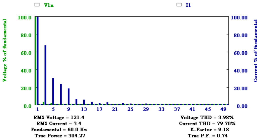
Figure 18 – Harmonic Levels after passing through 400 feet of 12 gauge wire
