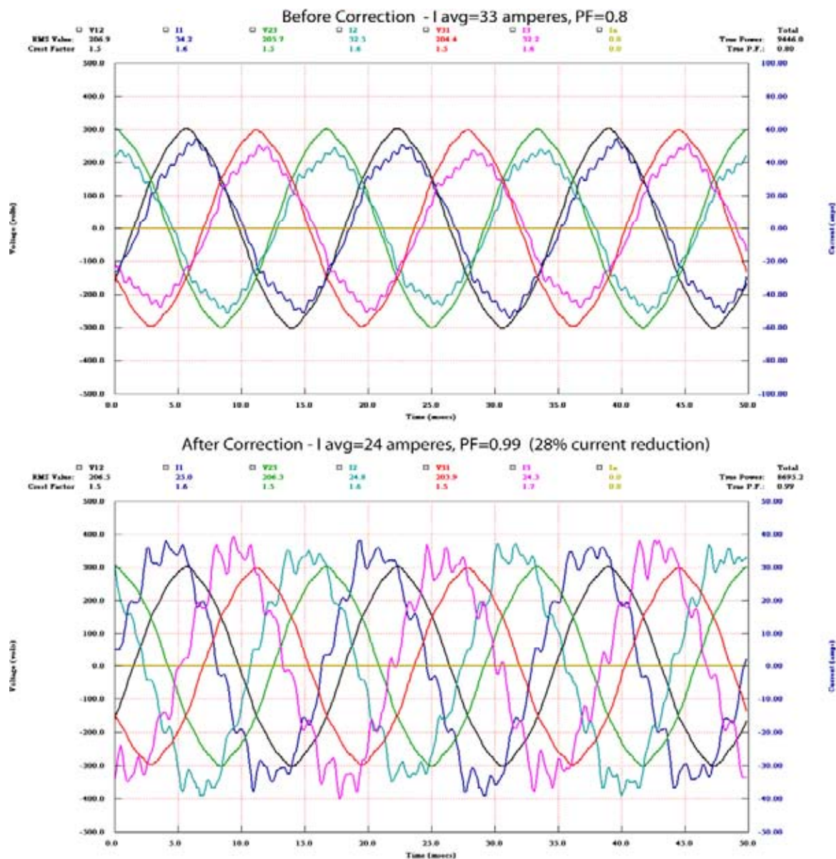
Figure 10 – Before and after waveforms for one of the seven compressors at the supermarket. I_{AVG} was reduced by 28% from 33 amperes to 24 amperes, while the power factor was raised from 0.8 to 0.99. That results in a 48% reduction in associated line losses.
